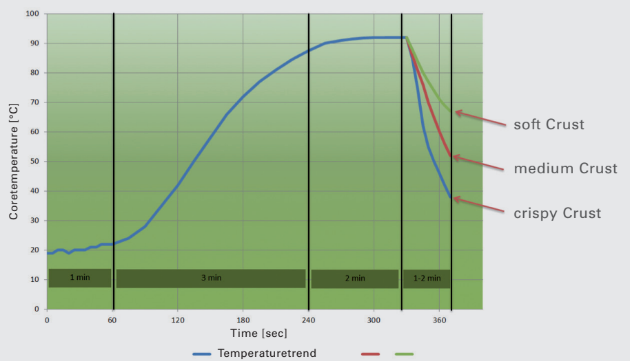
Core temperature trend at the vacuum baking process
